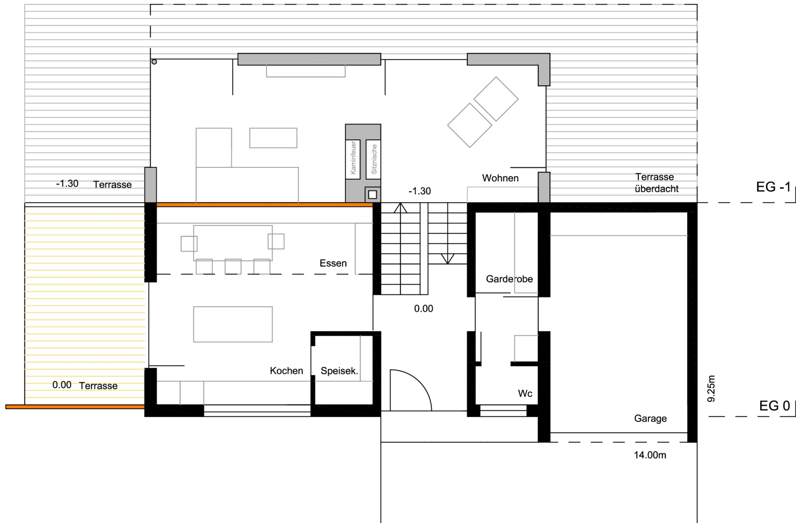
Hanggeschoss EG 0 / EG -1
